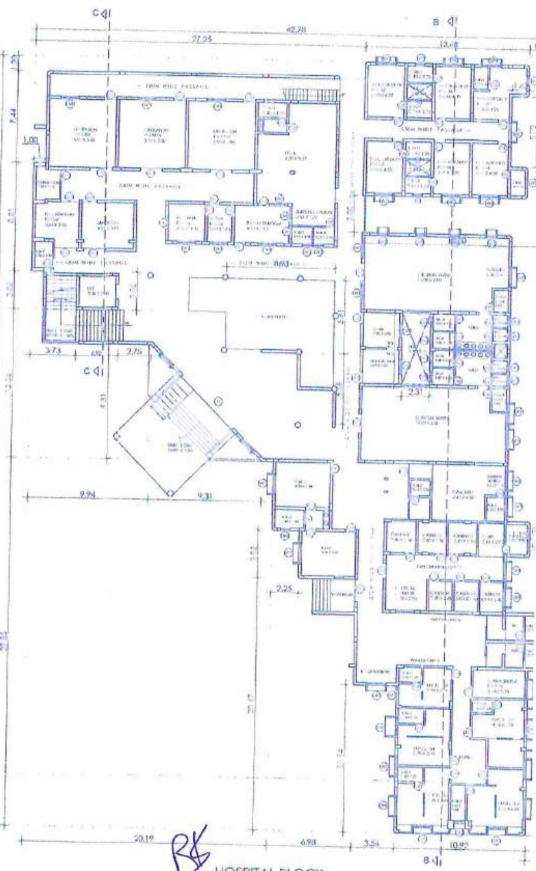
HOSPITAL BLOCK GROUND FLOOR PLAN
