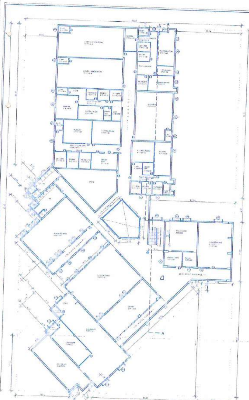
ACADEMIC BLOCK FIRST FLOOR PLAN (SCALE - 1:200)
